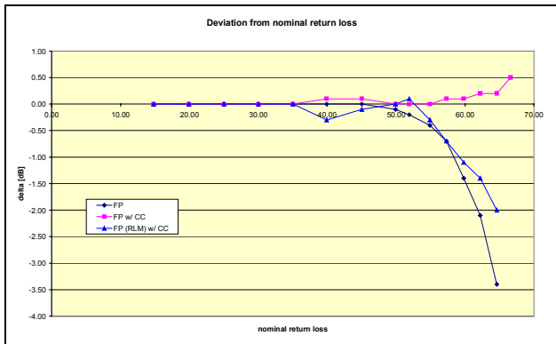
Figure 25: Deviation of measured Return Loss values from nominal Return Loss.
