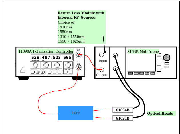
Figure 4: Components of the economic Optical Loss Analyzer Solution: Mainframe 8163B with Return Loss Module and Dual Channel Interface Module, Optical Heads and Polarization Controller.
