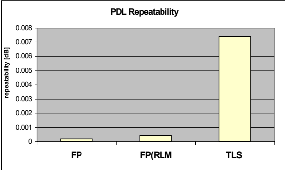
Figure 21: Repeatability of PDL measurements on a DUT with nominal PDL of 0.05\text{dB} \pm 0.02\text{dB} .
