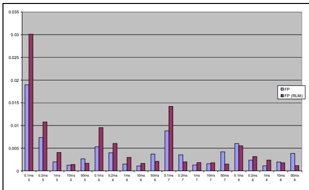
Figure 15: Repeatability of PDL measurement results, over different polarization scan rates and averaging times.
