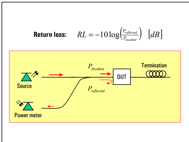
Figure 2: Return Loss - Definition and measurement principle.
