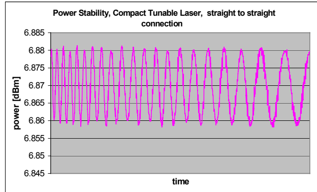
Figure 11: Power Stability measured with a straight to straight connection in the setup. The source is a tunable laser.
