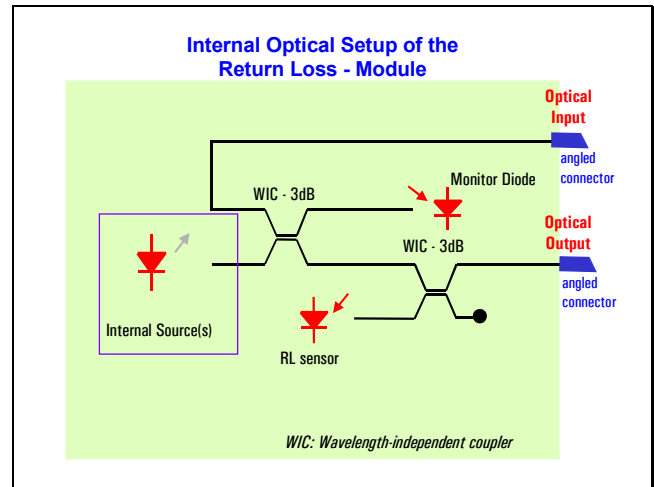
Figure 6: Optical Setup in the Return Loss Module.
