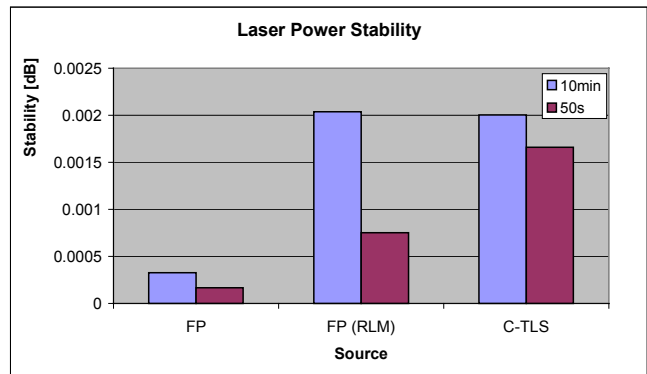
Figure 9: Long and Short Term Power Stability of various Sources.
