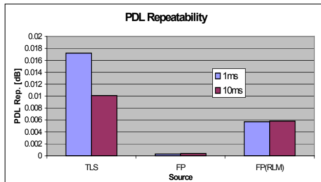
Figure 17: PDL repeatability for different sources.
