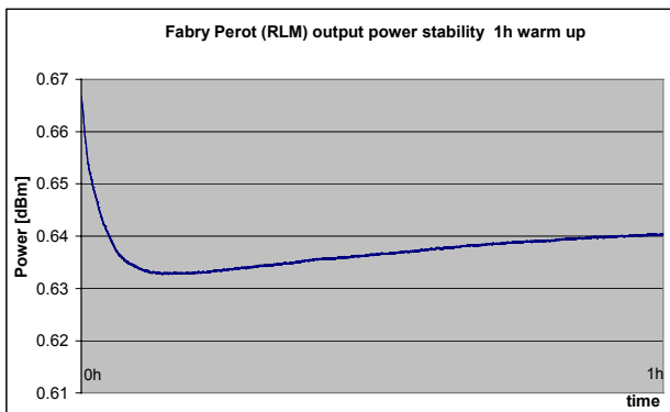
Figure 8: Output power of Fabry Perot Laser Source in Return Loss Module over 1hour during warm up time.
