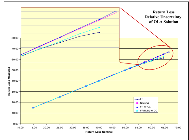
Figure 24: Return Loss Relative Uncertainty Measurement. The deviation from the nominal Return Loss gives an estimate for the uncertainty.
