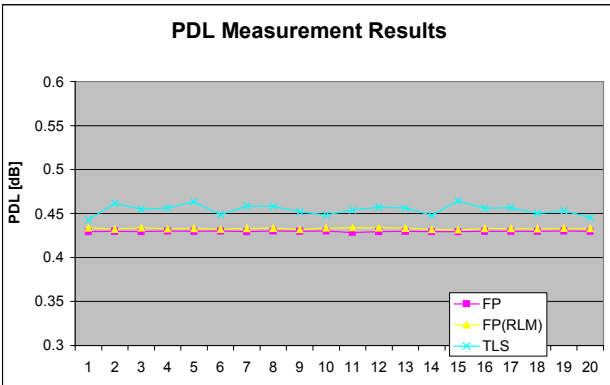
Figure 22: PDL measurement results with different sources on a DUT with nominal PDL of 0.45\text{dB} \pm 0.02\text{dB} .
