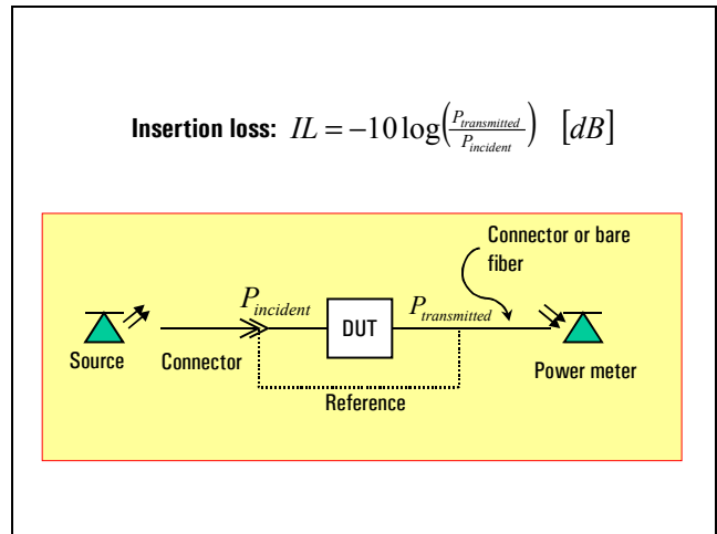
Figure 1: Insertion Loss - Definition and measurement principle.
