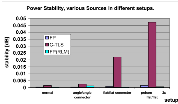
Figure 10: Influence of various setups on the power stability.
