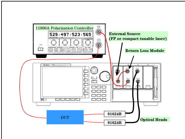
Figure 5: Components of the High-Performance / Tunable Optical Loss Analyzer solution.
