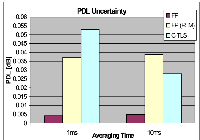
Figure 14: PDL uncertainty for different sources.
