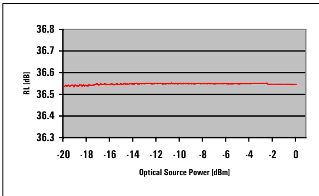
Figure 7: Monitoring the input power minimizes the impact of power fluctuations on return loss measurements.
