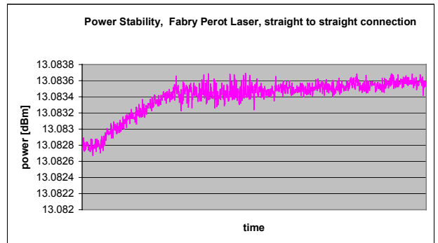
Figure 12: Power Stability measured with straight to straight connection in the setup. The source is a Fabry Perot Laser.
