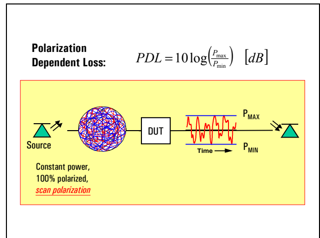
Figure 3: Polarization Dependent Loss - Definition and measurement principle.
