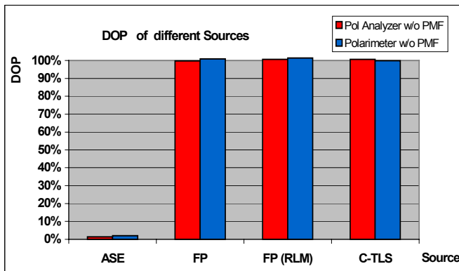
Figure 13: Degree of Polarization (DOP) for different sources.
