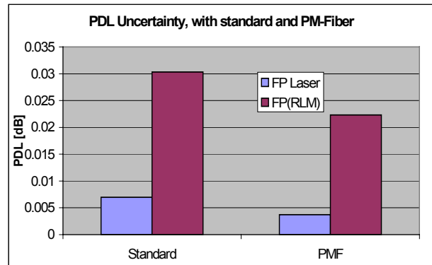
Figure 19: Comparison of the PDL uncertainty with and without using a polarization maintaining fiber (PMF) before the detector.
