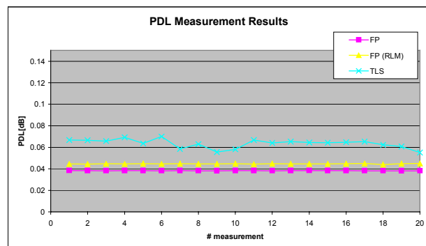
Figure 20: PDL measurement using different sources on a DUT with nominal PDL of 0.05\text{dB} \pm 0.02\text{dB} .
