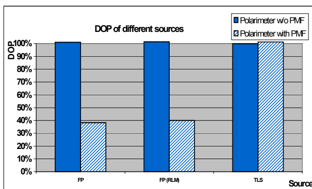
Figure 18: Depolarization of different sources using a polarization maintaining fiber.
