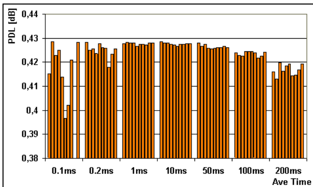
Figure 16: Repeatability of PDL measurements at scan rate 6 for different averaging times.
