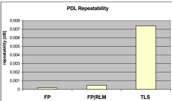
Figure 23: Repeatability of PDL measurements on a DUT with nominal PDL of 0.45\text{dB} \pm 0.02\text{dB} .
